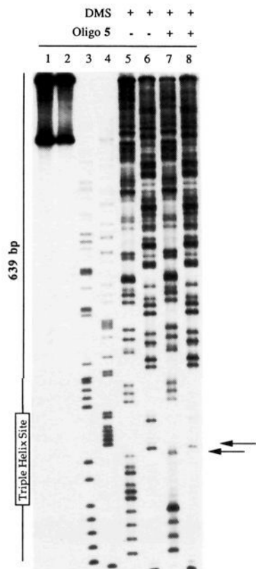
Figure 6. Autoradiogram of an 8% denaturing polyacrylamide gel used to separate DMS footprinting products. The reactions were carried out by incubating oligonucleotide 5 with the 3' end or 5' end ^{32}\text{P} labeled Hind III/Ssp I restriction fragment from plasmid pBCRI [ \sim 20\,000 cpm] in a solution of trisHCl (pH = 7.0, 40 mM), spermine (1.5 mM), NaCl (5 mM), \text{MgCl}_2 (10 mM), and \text{CaCl}_2 (10 mM) for 2 h at 24 °C. The reactions were initiated by the addition of dimethyl sulfate (DMS) (0.2% v/v) and allowed to proceed for 90 s at 24 °C. The reactions were stopped as described by Maxam and Gilbert. 14 The DNA was precipitated with ethanol, redissolved in 50 \mu\text{L} of 10% aqueous piperidine, and heated at 90 °C for 30 min. Concentrations listed are final concentrations. The solutions were lyophilized and the cleavage products were analyzed by gel electrophoresis. Odd numbered lanes contain 5' end labeled fragment, even numbered lanes contain 3' end labeled fragment. (Lanes 1 and 2) Intact labeled fragment in the absence of oligonucleotide 5 and DMS. (Lanes 3 and 4) Products of adenine-specific sequencing reactions. 15 (Lanes 5 and 6) Cleavage products generated in the presence of DMS in the absence of oligonucleotide 5. (Lanes 7 and 8) Cleavage products generated in the presence of DMS and 10 \mu\text{M} oligonucleotide 5. Arrows indicate guanines in the binding site not protected by oligonucleotide 5.
