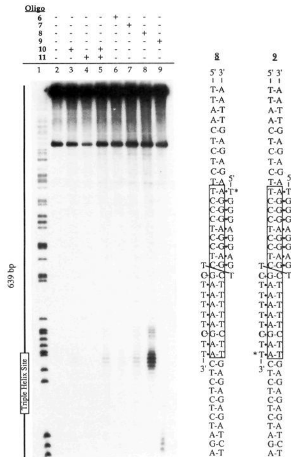
Figure 9. (Left) Autoradiogram of an 8% denaturing polyacrylamide gel used to separate affinity cleavage products. The cleavage reactions were carried out by combining a mixture of oligonucleotide-EDTA (200 nM) and Fe(NH 4 ) 2 (SO 4 ) 2 ·6H 2 O (500 nM) with the 5' end 32 P labeled Hind III/Ssp I restriction fragment from plasmid pPBCRII [ \sim 15 000 cpm] in a solution of tris acetate (pH = 7.0, 50 mM), spermine (1 mM), NaCl (10 mM), and calf thymus DNA (0.1 mM bp) and then incubating for 1 h at 37 °C. The reactions were initiated by the addition of dithiothreitol (DTT) (4 mM) and allowed to proceed for 18 h at 37 °C. Concentrations listed are final concentrations. The DNA was precipitated with ethanol and the cleavage products were analyzed by gel electrophoresis. (Lane 1) Products of an adenine-specific sequencing reaction. 15 (Lane 2) Intact 5' labeled fragment obtained after incubation under the conditions of the cleavage reactions in the absence of oligonucleotide-EDTA-Fe II . (Lanes 3-9) DNA cleavage products produced by oligonucleotide-EDTA-Fe II 6-11: 10 (lane 3); 11 (lane 4); 10 + 11 (200 nM each) (lane 5); 6 (lane 6); 7 (lane 7); 8 (lane 8); 9 (lane 9). (Right) Sequences of triple helical complexes formed between oligonucleotides 8 and 9 and the 5'-(Py) 3 (Pu) 3 -3' target site.
