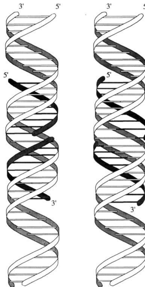
Figure 13. (Left) Ribbon model depicting 9-mer oligonucleotides binding to adjacent triple helix sites for the sequence 5'-(Pu) 9 (Py) 9 -3'. The 3' end of one binding site appears to overlap with the 5' end of the adjacent site in the major groove. (Right) Ribbon model depicting 9-mer oligonucleotides binding to adjacent triple helix sites for the sequence 5'-(Py) 9 (Pu) 9 -3'. No binding site overlap is apparent in the major groove.
