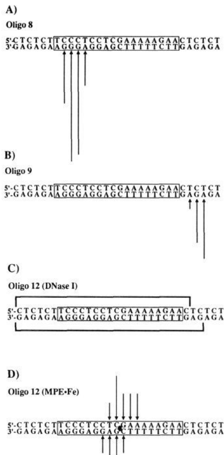
Figure 12. (A) Cleavage pattern generated by oligonucleotide 8. The box indicates the double stranded sequence bound. Positions of the arrows show the sites of cleavage and heights indicate extent of cleavage at that site. (B) Cleavage pattern generated by oligonucleotide 9. (C) DNase I footprint generated by oligonucleotide 12. Bases within the brackets are protected from cleavage by DNase I. (D) MPE-Fe II reactivity within the target site bound by oligonucleotide 12. Arrows indicate positions of increased cleavage upon binding. Arrow heights indicate the extent of cleavage at that site. The dark circle indicates the intercalation site.
