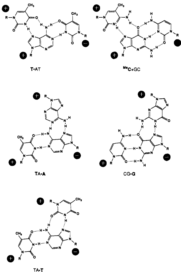
Figure 2. Models for base triplets formed when an oligonucleotide binds in the major groove and simultaneously recognizes both strands. All bases are in the anti conformation. (+) and (-) indicate relative orientations of the phosphate-deoxyribose backbone.
