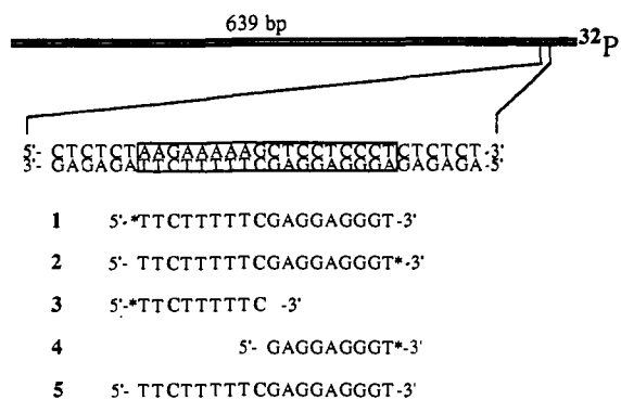
Figure 3. The duplex target site present on the 639 bp Hind III/Ssp I restriction fragment from plasmid pPBCRI containing two 9-mer purine tracts on alternate strands joined at a 5'-PuPy-3' junction. The double stranded region bound in the triple helix is boxed. The sequences of oligonucleotide-EDTA's 1-5 are shown, where T* indicates the position of thymidine-EDTA and bold type C indicates 5-methyldeoxycytidine.
