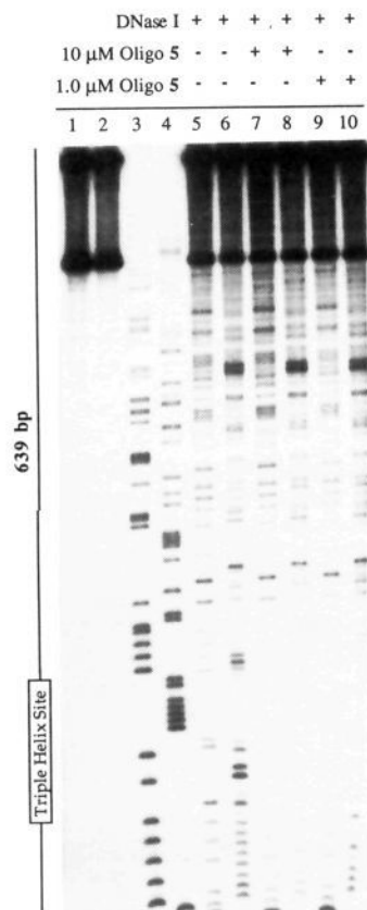
Figure 5. Autoradiogram of an 8% denaturing polyacrylamide gel used to separate DNase I footprinting products. The cleavage reactions were carried out by incubating oligonucleotide 5 with the 3' end or 5' end ^{32}\text{P} labeled Hind III/Ssp I restriction fragment from plasmid pPBCRI [ \sim 20\,000 cpm] in a solution of trisHCl (pH = 7.0, 40 mM), spermine (1.5 mM), NaCl (5 mM), \text{MgCl}_2 (10 mM), and \text{CaCl}_2 (10 mM) for 2 h at 24 °C. The reactions were initiated by the addition of nonspecific single stranded oligonucleotide (1 μM) and DNase I (0.25 units/μL) and allowed to proceed for 10 min at 24 °C. The reactions were stopped by the addition of calf thymus DNA (0.1 μM bp) and EDTA (50 mM). Concentrations listed are final concentrations. The DNA was precipitated with ethanol and the cleavage products were analyzed by gel electrophoresis. Odd numbered lanes contain 5' end labeled fragment and even numbered lanes contain 3' end labeled fragment. (Lanes 1 and 2) Intact labeled fragment in the absence of oligonucleotide 5 and DNase I. (Lanes 3 and 4) Products of adenine-specific sequencing reactions. 15 (Lanes 5 and 6) DNase I cleavage products in the absence of oligonucleotide 5. (Lanes 7 and 8) DNase I cleavage products in the presence of 10 μM oligonucleotide 5. (Lanes 9 and 10) DNase I cleavage products in the presence of 1 μM oligonucleotide 5.
