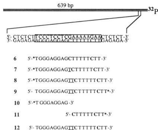
Figure 8. The duplex target site present on the 639 bp Hind III/Ssp I restriction fragment from plasmid pPBCRII containing two 9-mer purine tracts on alternate strands joined at a 5'-PyPu-3' junction. The double stranded region bound in the triple helix is boxed. The sequences of oligonucleotide-EDTA's 6-12 are shown, where T* indicates the position of thymidine-EDTA, bold type C indicates 5-methyldeoxycytidine, and the underlined thymidines indicate the linker domain.
