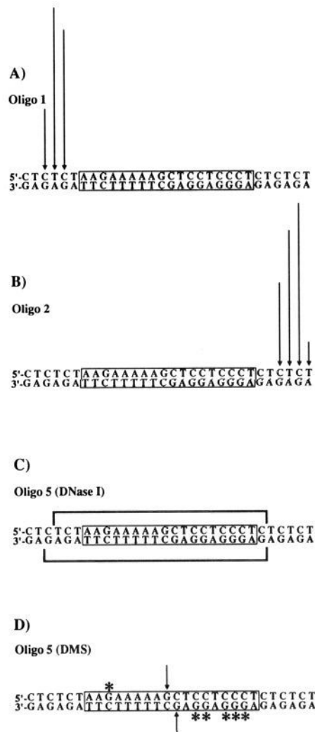
Figure 7. (A) Cleavage pattern generated by oligonucleotide 1. The box indicates the double stranded sequence bound. Positions of the arrows show the sites of cleavage and heights indicate extent of cleavage at that site. (B) Cleavage pattern generated by oligonucleotide 2. (C) DNase I footprint generated by oligonucleotide 5. Bases within the brackets are protected from cleavage by DNase I. (D) Dimethyl sulfate (DMS) reactivity within the target site bound by oligonucleotide 5. Asterisks (*) indicate bases within the binding site protected from methylation by DMS. Arrows indicate bases within the binding site which remain reactive to DMS upon binding of oligonucleotide 5.
