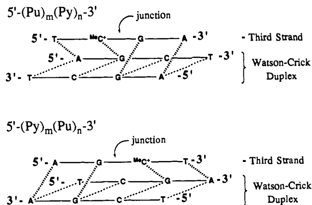
Figure 1. Models representing oligonucleotides binding in the major groove and simultaneously recognizing both strands of the duplex by forming hydrogen bonds to the purine in a WC base pair. Base triplet specificities and required strand orientations are maintained by alternating between triple helix motifs at junctions between purines and pyrimidines on one strand of the duplex. (Above) Triple helix formed at a 5'-(Pu) m (Py) n -3' target site. (Below) Triple helix formed at a 5'-(Py) m (Pu) n -3' target site.
