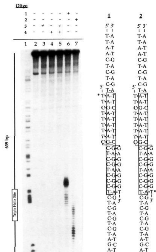
Figure 4. (Left) Autoradiogram of an 8% denaturing polyacrylamide gel used to separate affinity cleavage products. The cleavage reactions were carried out by combining a mixture of oligonucleotide-EDTA (200 nM) and \text{Fe}(\text{NH}_4)_2(\text{SO}_4)_2 \cdot 6\text{H}_2\text{O} (500 nM) with the 3' end ^{32}\text{P} labeled Hind III/Ssp I restriction fragment from plasmid pPBCRI [ \sim 15\,000 cpm] in a solution of tris acetate, pH = 7.0 (50 mM), spermine (1 mM), NaCl (10 mM), and calf thymus DNA (0.1 mM bp) and then incubating for 1 h at 37 °C. Concentrations listed are final concentrations. The reactions were initiated by the addition of dithiothreitol (DTT) (4 mM) and allowed to proceed for 18 h at 37 °C. The DNA was precipitated with ethanol and the cleavage products were analyzed by gel electrophoresis. (Lane 1) Products of an adenine-specific sequencing reaction. 15 (Lane 2) Intact 3' labeled fragment obtained after incubation under the conditions of the cleavage reactions in the absence of oligonucleotide-EDTA- \text{Fe}^{\text{II}} . (Lanes 3-7) DNA cleavage products produced by oligonucleotide-EDTA- \text{Fe}^{\text{II}} 1-4: 3 (lane 3); 4 (lane 4) 3 + 4 (200 nM each) (lane 5); 1 (lane 6); 2 (lane 7). (Right) Sequences of triple helical complexes formed between oligonucleotides 1 and 2 and the 5'-(Pu) 9 -(Py) 9 -3' target site.
