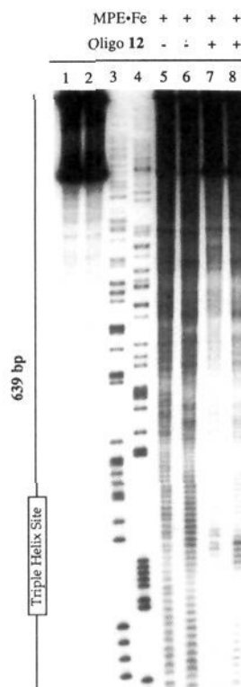
Figure 11. Autoradiogram of an 8% denaturing polyacrylamide gel used to separate MPE-Fe footprinting products. The cleavage reactions were carried out by incubating oligonucleotide 12 with the 3' end or 5' end ^{32} P labeled Hind III/Ssp I restriction fragment from plasmid pBCR11 [ \sim 20\,000 cpm] in a solution of trisHCl (pH = 7.0, 40 mM), spermine (1.5 mM), NaCl (5 mM), MgCl 2 (10 mM), and CaCl 2 (10 mM) for 2 h at 24 °C. The reactions were initiated by the addition of MPE-Fe (5 \mu M) and DTT (4 mM) and allowed to proceed for 5 min at 24 °C. Concentrations listed are final concentrations. The reactions were stopped by precipitation with ethanol and the cleavage products were analyzed by gel electrophoresis. Odd numbered lanes contain 5' end labeled fragment, even numbered lanes contain 3' end labeled fragment. (Lanes 1 and 2) Intact labeled fragment in the absence of oligonucleotide 12 and MPE-Fe. (Lanes 3 and 4) Products of adenine-specific sequencing reactions. 15 (Lanes 5 and 6) MPE-Fe cleavage products in the absence of oligonucleotide 12. (Lanes 7 and 8) MPE-Fe cleavage products in the presence of 10 \mu M oligonucleotide 12. Bracket indicates bases in the binding site hyperreactive to MPE-Fe.
