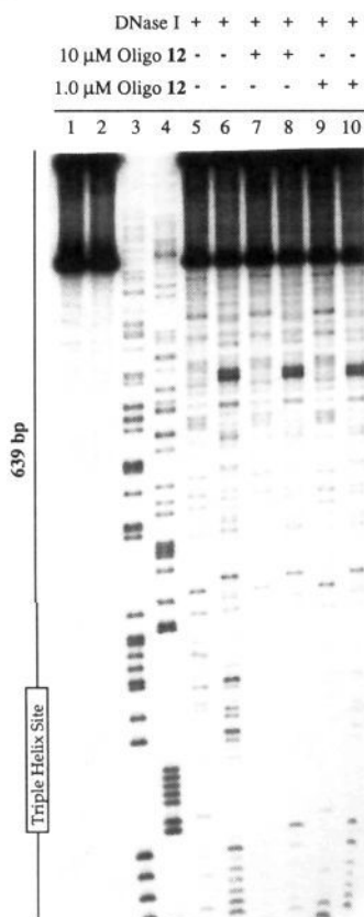
Figure 10. Autoradiogram of an 8% denaturing polyacrylamide gel used to separate DNase I footprinting products. The cleavage reactions were carried out by incubating oligonucleotide 12 with the 3' end or 5' end ^{32} P labeled Hind III/Ssp I restriction fragment from plasmid pBCR11 [ \sim 20\,000 cpm] in a solution of trisHCl (pH = 7.0, 40 mM), spermine (1.5 mM), NaCl (5 mM), MgCl 2 (10 mM), and CaCl 2 (10 mM) for 2 h at 24 °C. The reactions were initiated by the addition of nonspecific single stranded oligonucleotide (1 \mu M) and DNase I (0.25 units/ \mu L) and allowed to proceed for 10 min at 24 °C. The reactions were stopped by the addition of calf thymus DNA (0.1 \mu M bp) and EDTA (50 mM). Concentrations listed are final concentrations. The DNA was precipitated with ethanol and the cleavage products were analyzed by gel electrophoresis. Odd numbered lanes contain 5' end labeled fragment, even numbered lanes contain 3' end labeled fragment. (Lanes 1 and 2) Intact labeled fragment in the absence of oligonucleotide 12 and DNase I. (Lanes 3 and 4) Products of adenine-specific sequencing reactions. 15 (Lanes 5 and 6) DNase I cleavage products in the absence of oligonucleotide 12. (Lanes 7 and 8) DNase I cleavage products in the presence of 10 \mu M oligonucleotide 12. (Lanes 9 and 10) DNase I cleavage products in the presence of 1 \mu M oligonucleotide 12.
